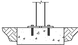
SURFACE MOUNT DETAIL
