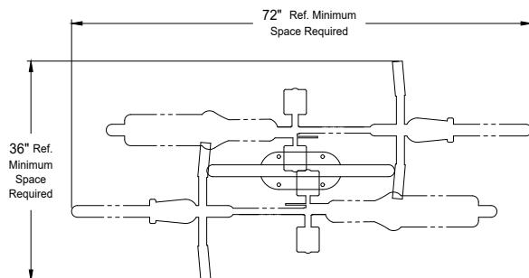
Top View Showing Recommended Spacing Requirements (1/2 Scale)
