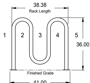
Model: 850602 2-Hump 5 Bike Capacity
