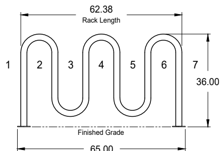
Model: 850603 3-Hump 7 Bike Capacity
