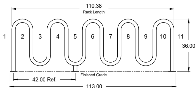
Model: 850605 5-Hump 11 Bike Capacity
