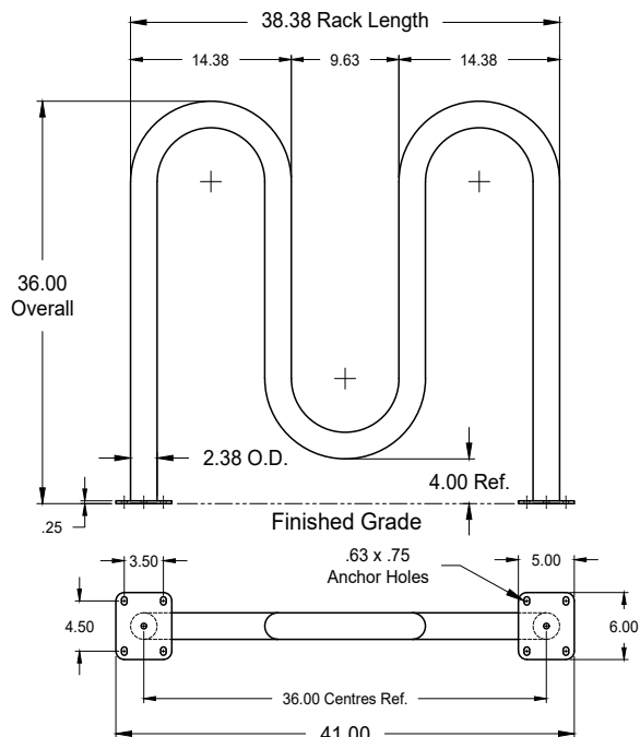
Model: 850602 2-Hump, Surface Mount
