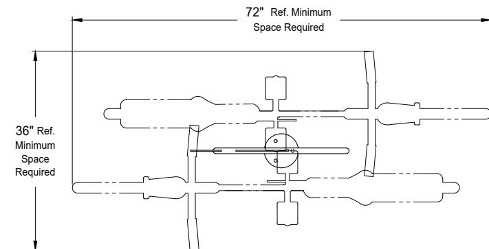
Top View Showing Recommended Spacing Requirements
