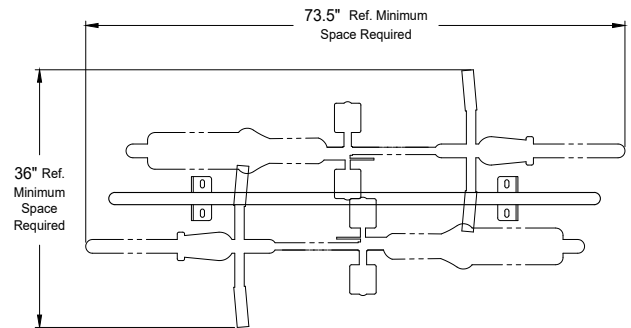
Top View Showing Recommended Spacing Requirements Rack Capacity: 2 Bikes (1/2 Scale)
